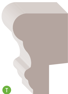
90850 1-3/16" x 1-3/4" (3/8" Offset) PLDF 16'
