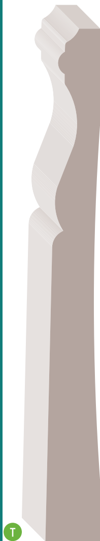
10673 9/16" x 5-3/16"
