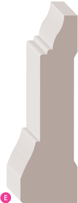
00738 1" x 3-1/4"
