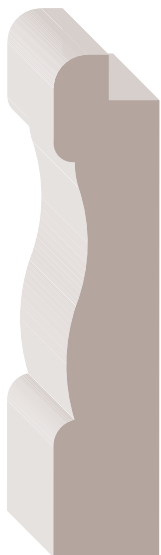
WCB01 Wainscot Cap & Base 9/16" x 2-5/8" (17/64" Offset)
