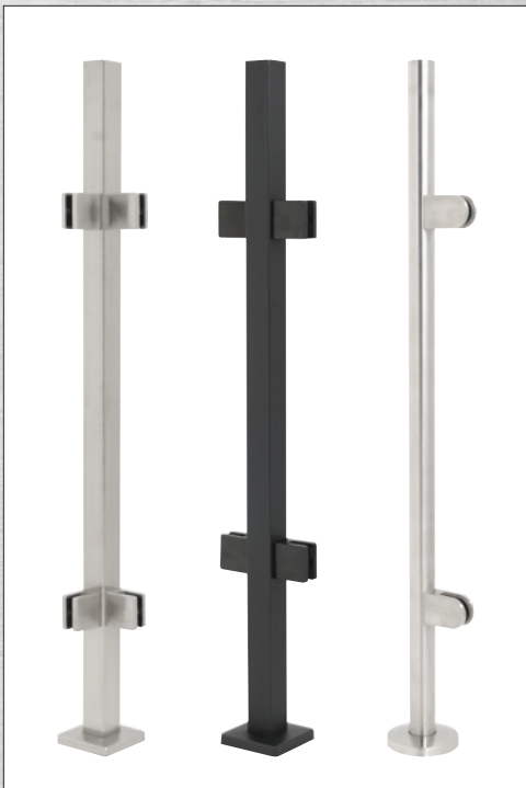
Square, pre-drilled post 9421 and 9422, cover flange 9402, glass clip S7340SB-B, top mount brackets 9601 and 9603, round tube 9010 and end cap 9254
